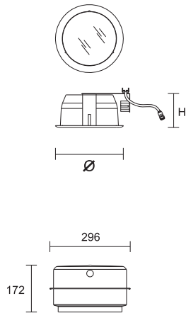
art. 2973 Ugradna kutija za montažu u beton Integrated box to be installed into concrete
