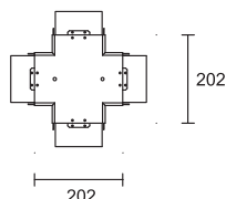
Spoj na četiri strane Four-side connection art.9476
