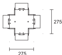
Spoj na četiri strane Four-side connection art.9477
