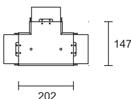
Spoj na tri strane T Tree-side connection T art.9473
