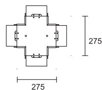
Spoj na četiri strane Four-side connection art.9475
