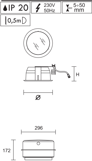
art. 2973 Ugradna kutija za montažu u beton Integrated box to be installed into concrete
